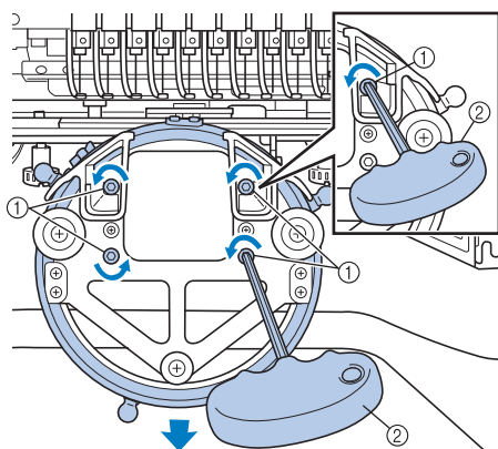
① Hexagonal screws ② Allen screwdriver (large) → When the screws are loosened, the ring can be lowered.
