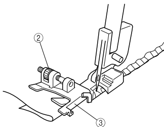
② Adjusting screw ③ Fabric guide
