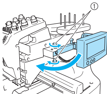
① Thumb screws
