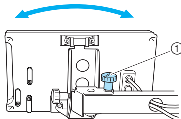
① Thumb screw
