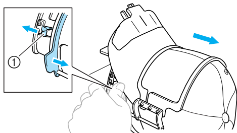
① Holder
