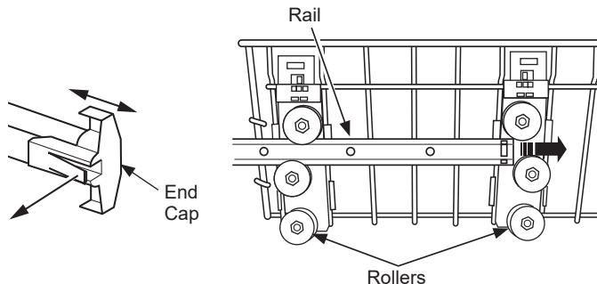
Upper Rack
