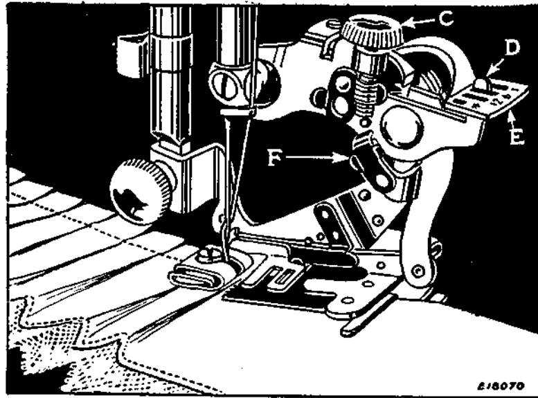
FIG. 69. PLAITHING WITH THE RUFFLER
