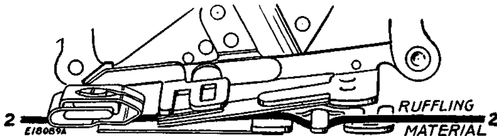
FIG. 70. CORRECT POSITION FOR THE MATERIAL
