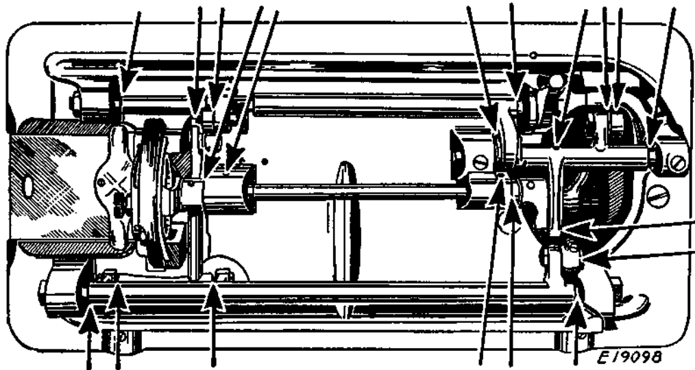
FIG. 29. OILING POINTS IN BASE OF MACHINE
