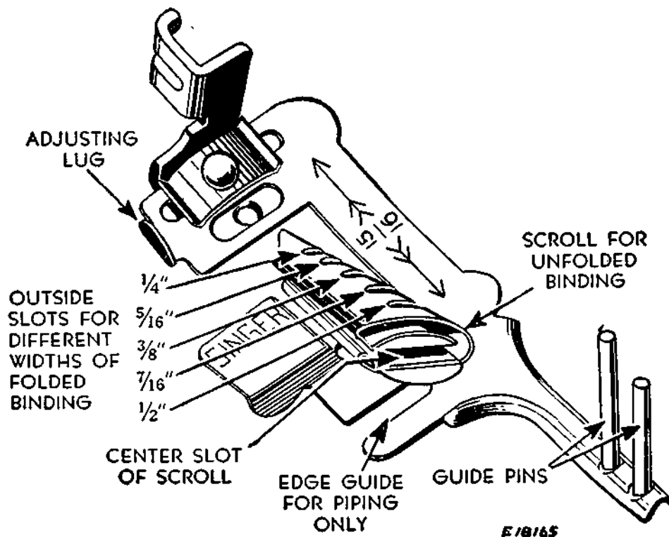
FIG. 44. MULTIPLE SLOTTED BINDER 160359
