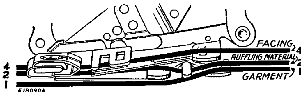
FIG. 65. CORRECT POSITIONS FOR THE MATERIALS
