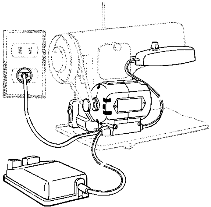
FIG. 148. PORTABLE MACHINE WITH FOOT CONTROL.
