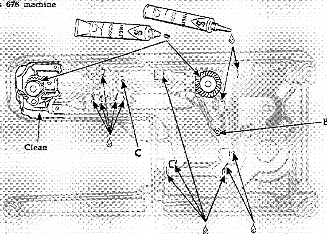
Class 676 machine
