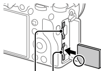
Ranhura 2 Ranhura 1
