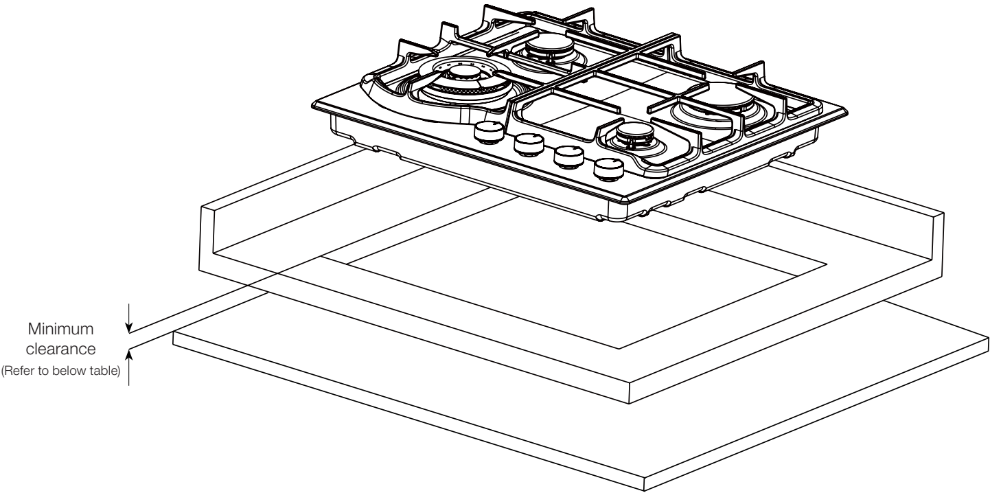
Figure 5e - Clearance from bench to cupboard
