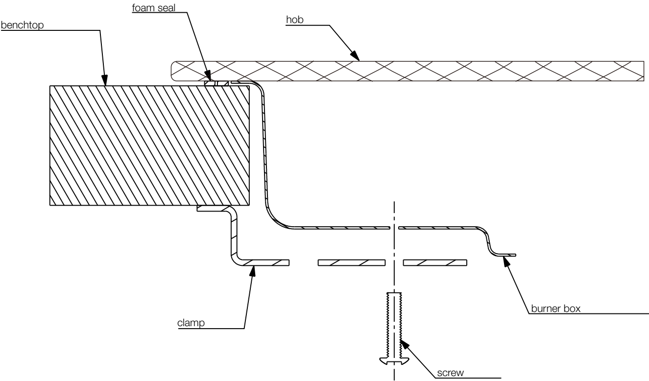
Figure 7 – Clamp fitment
