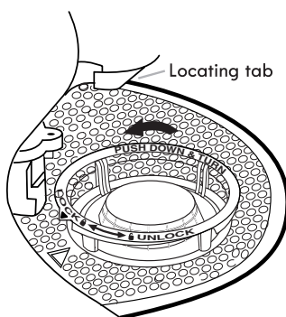
To remove Upper Filter Assembly
