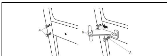
A. 5/16" Hex-head hinge screws B. Washers
